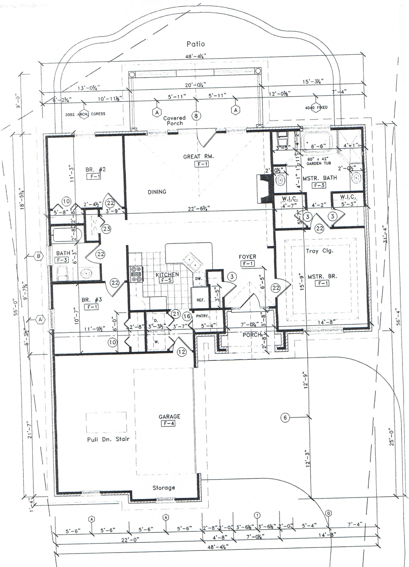
A37 First Floor Plan 1488 S.F. Homes of Chadsworth 4/21/9
