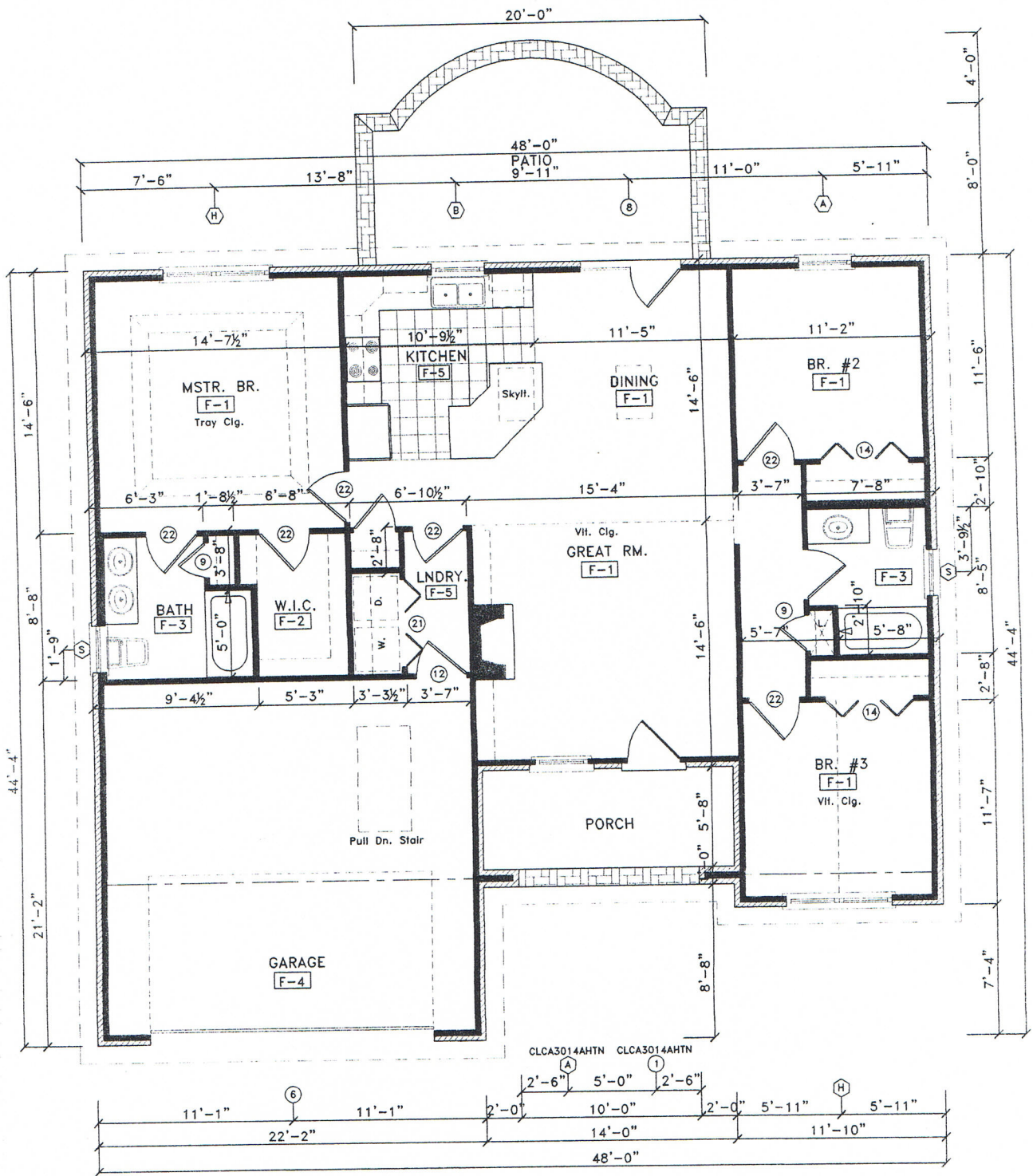
A22 First Floor Plan 1323 S.F. Homes of Chadsworth 4/17/9
