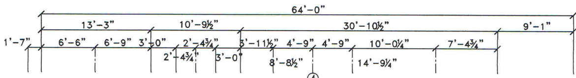
C29 Front Elevation Homes of Chadsworth
