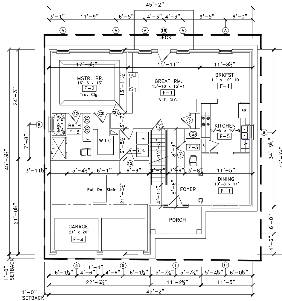
CW First Floor Plan A-30 1304 S.F. 9/15/10
